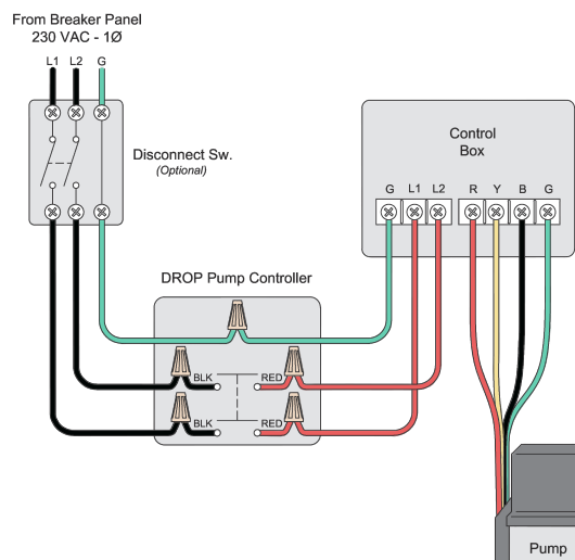
230VAC 3-Wire Pump Wiring Diagram (P/Ns: B-PC230-25, B-PC230-30)
